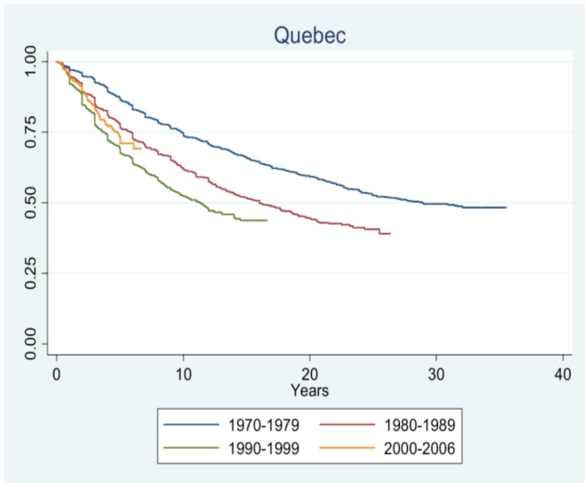
Figure 3. Union Dissolution in Québec, by Cohort of Union Formation
