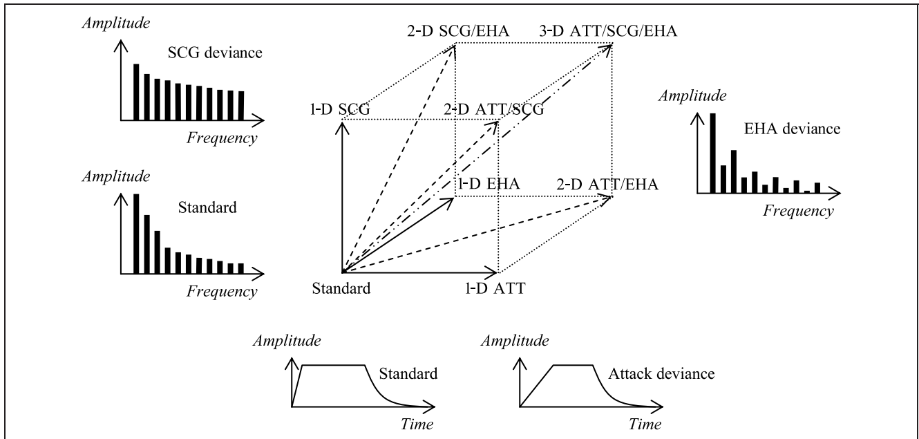
Figure 1. Stimulus construction. All stimuli have the same pitch, loudness, and perceived duration but vary along three timbral dimensions. ATT = attack time; SCG = spectral center of gravity; EHA = even-harmonic attenuation. The edges of the stimulus cube represent equal perceived dissimilarity. Arrows represent the seven timbre changes from the standard, with solid lines for unidimensional (1-D) deviants and dashed lines for multidimensional (2-D and 3-D) deviants.
