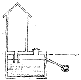
Aquaprivy
