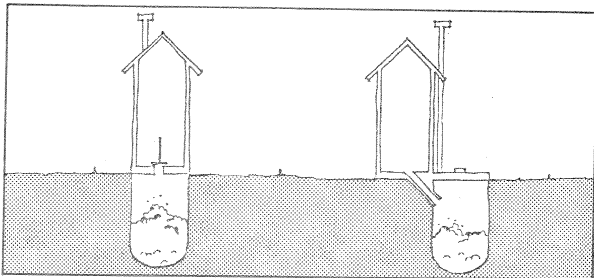
PIT LATRINES
