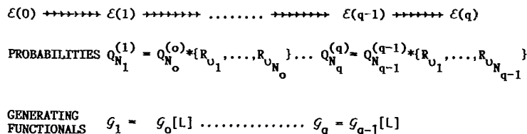
FIG. 1. Diagrammatic representation of the evolution of the population from generation to generation. \mathcal{E}(q') , q' = 0, 1, \dots, q , represents the population from the q' th generation, q' = 0, 1, \dots, q , and the arrow represents the process of replacement of the components from a generation by their direct offspring, expressed by the convolution product in the (N, \mathbf{r}_1, \dots, \mathbf{r}_N) space or by the process of functional iteration in the space of test functions W(\mathbf{r}) .
