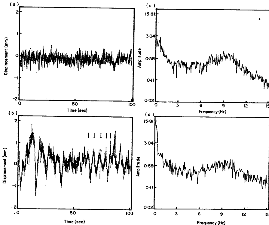
FIG. 5. (a), (b). Time series of the displacement of the index finger of a healthy subject (subject IT) performing the delayed visual tracking task described in the text with an added time delay of (a) 300 msec and (b) 1500 msec. The amplitude of the displacements in finger position increases with the time delay and in the case of the 1500 msec delay a regular low frequency oscillation appears intermittently (indicated by ↓). In (c) and (d) the power spectra of the finger displacement time series shown, respectively, in (a) and (b) is plotted for frequencies from 0-15 Hz. The logarithm of the amplitude of the power spectrum has been plotted in arbitrary units. With increasing delay, more power appears at frequencies < 1.5 Hz.
