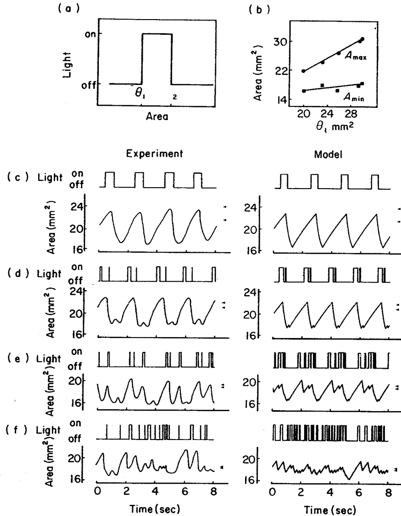
FIG. 3. Comparison of the changes in pupil area that occur as a function of time with imposed mixed feedback to those predicted by eqn (3) (subject JM). The piecewise constant mixed feedback is shown in (a). The parameter \alpha_c = 3.88 \text{ sec}^{-1} , \alpha_d = 0.265 \text{ sec}^{-1} , A_{on} = 15.5 \text{ mm}^2 , A_{off} = 34.2 \text{ mm}^2 were measured in a preliminary experiment with piecewise constant negative feedback as discussed in the legend to Fig. 2 [data shown in (b)] and \tau was 411 msec. The upper ( \theta_2 ) and lower ( \theta_1 ) area thresholds have been indicated by the " \blacktriangleleft " at the right hand sides of the figure and were respectively: (c) 21.5 mm 2 , 24.5 mm 2 ; (d) 21 mm 2 , 22 mm 2 ; (e) 18.9 mm 2 , 19.5 mm 2 ; (f) 17.95 mm 2 , 18.5 mm 2 .
