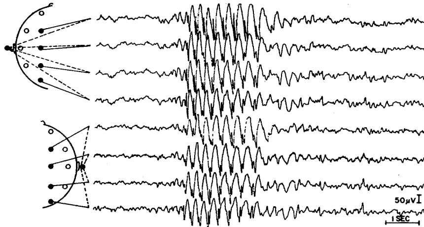
FIG. 1. Electroencephalographic recording (EEG) of a train of generalized 3 Hz spike and wave discharges in patient with a history of absence attacks and generalized tonic-clonic seizures. Note the abrupt change in the frequency and morphology of the EEG that is associated with the onset and offset of this train. (From Spehlmann, 1985, with permission from the publisher.)
