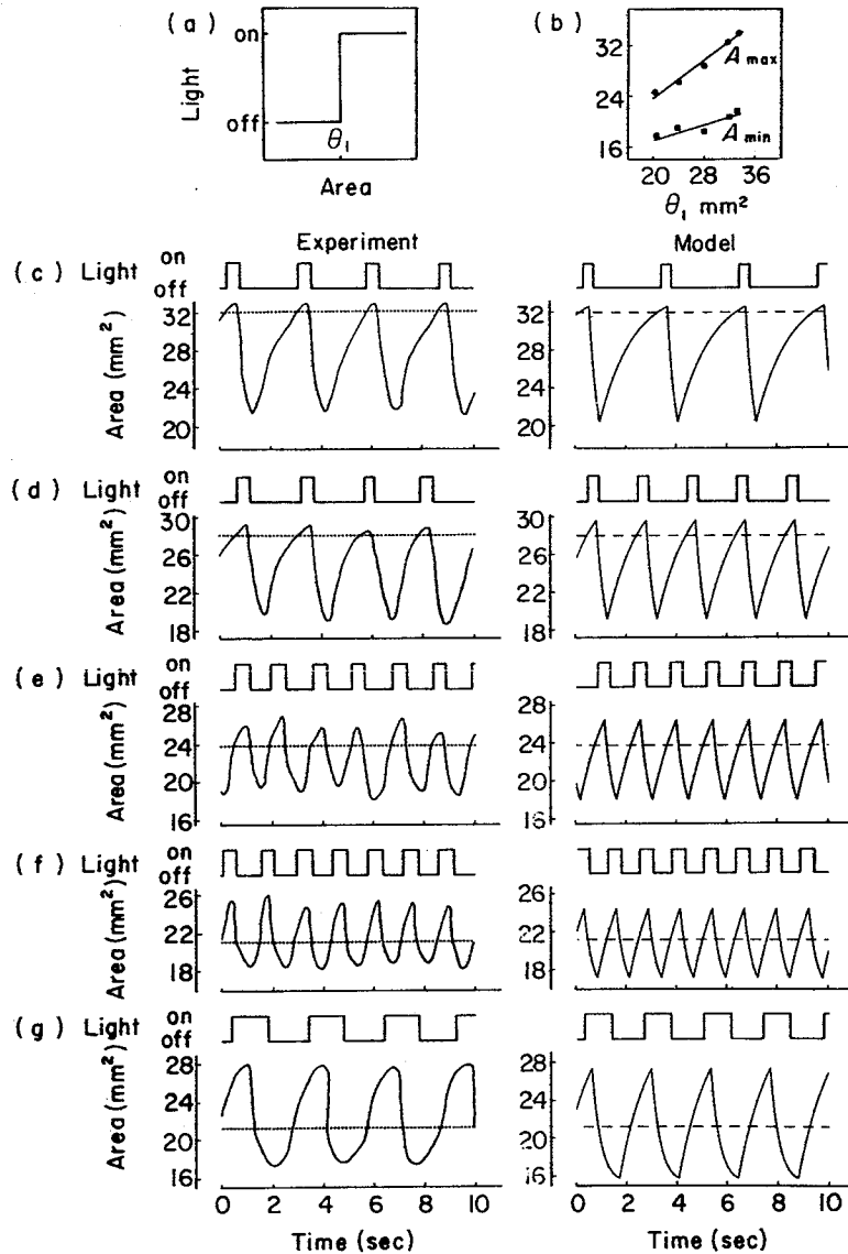
FIG. 2. Comparison of the changes in pupil area that occur as a function of time with imposed negative feedback to those predicted by eqn (2) (subject MC). The piecewise constant negative feedback is shown in (a). The pupil latency time was 285 msec. In (c-f) the machine delay was 100 msec ( \tau = 385 msec) and in (g) the machine delay was increased to 579 msec ( \tau = 864 msec). The area threshold, \theta_1 , was set at: (c) 32 mm 2 , (d) 28.1 mm 2 , (e) 23.8 mm 2 , and 21.4 mm 2 in (f) and (g). For negative feedback, it can be shown (an der Heiden & Mackey, 1982; Milton & Longtin, unpublished results) that A_{max} = \theta_1 \exp(-\alpha_d \tau) + A_{on} [1 - \exp(-\alpha_d \tau)] and A_{min} = \theta_1 \exp(-\alpha_c \tau) + A_{on} [1 - \exp(-\alpha_c \tau)] , where A_{max} , A_{min} are, respectively, the maximum and minimum amplitudes of the pupil area oscillations. The values of \alpha_c , A_{on} , \alpha_d , A_{off} used to calculate the solutions of eqn (2) were calculated from plots of A_{min} , A_{max} vs. \theta_1 shown in (b) and were \alpha_c = 3.11 \text{ sec}^{-1} , \alpha_d = 0.74 \text{ sec}^{-1} , A_{on} = 15.7 \text{ mm}^2 , A_{off} = 34.5 \text{ mm}^2 . In (b) the values of A_{max} , A_{min} represent values averaged over a minimum of ten consecutive cycles.
