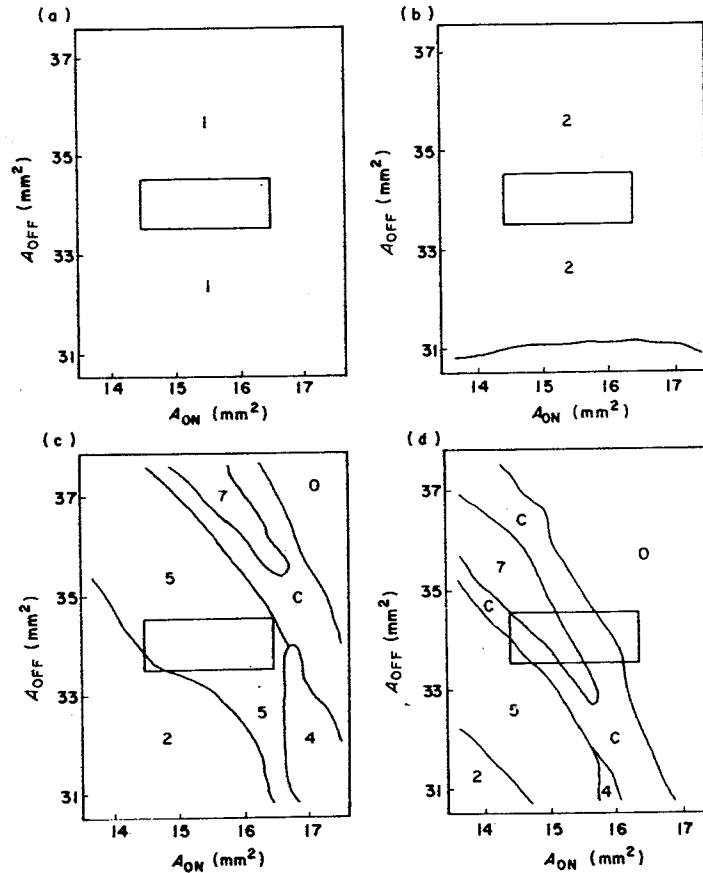
FIG. 4. The (A_{on}, A_{off}) -parameter space for eqn (3) for the values of the area thresholds \theta_1, \theta_2 in Fig. 3 [(a), (b), (c), and (d) correspond, respectively, to Figs 3(c), (d), (e), and (f).] In constructing these parameter spaces the values of \alpha_c, \alpha_d, \tau have been fixed and we have classified the periodic solutions of eqn (3) symbolically by the number of light pulses per period [i.e. Fig. 3(d) shows a type 2 solution since there are two light pulses per period]. The region labelled "C" contains very complex periodic solutions in close proximity as well as unstable mixing solutions. The rectangular boxes enclose the measured values of A_{on}, A_{off} ( \geq 10 consecutive values). Since in eqn (3), constriction and dilation occur as first order processes, it is possible to measure the values of A_{on}, A_{off} cycle to cycle using the values of, respectively, \alpha_c, \alpha_d (Longtin & Milton, 1988).
