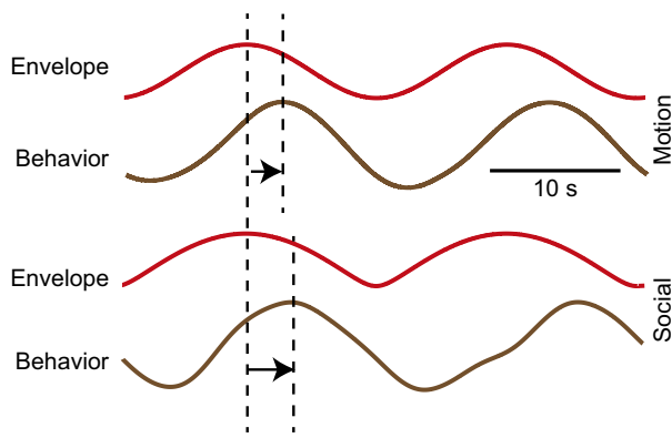
Fig. 9. Comparing behavioral responses to motion and social envelopes. Top: 0.05 Hz motion envelope waveform (red) and EOD frequency response (brown). Note that the behavioral response lags the stimulus (dashed vertical lines). Bottom: same, but for an example 0.05 Hz social envelope. Note the increased response lag.
