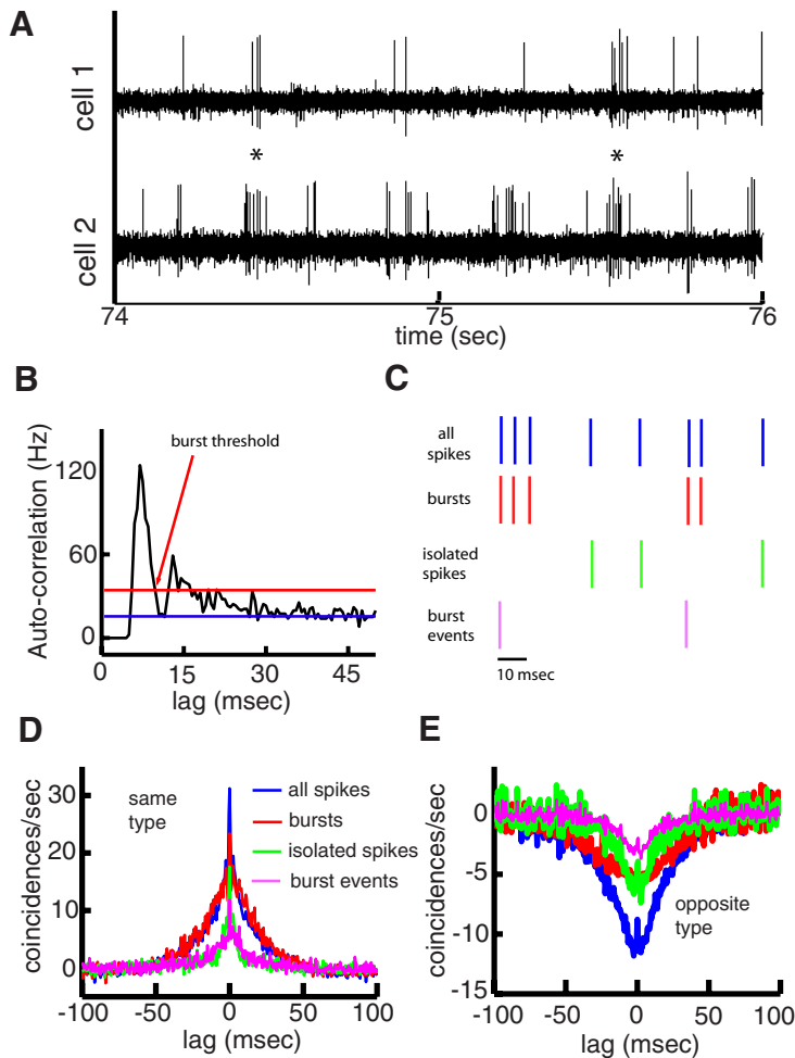
FIG. 2. Pyramidal cell activity consists of correlated bursts. A : extracellular recording from a pair of I-type pyramidal cells. B : auto-correlogram of an example cell with expected value from a Poisson process (blue) and 99.9% confidence interval (red). The burst threshold value is indicated by the arrow. C : illustration of the procedure used to separate the spike train (blue) into bursts (red), isolated spikes (green), and burst events (purple) using the interspike interval (ISI) threshold determined. If n consecutive ISIs are all smaller than the burst threshold, then all associated spikes are considered to be part of the burst. The remaining spikes are considered isolated spikes. Burst events are obtained by taking only the 1st spike of each burst. D : population-averaged ( n = 75 ) CCGs obtained from the full spike trains (blue), burst spike trains (red), isolated spike trains (green), and burst event spike trains (purple) for same-type pyramidal cell pairs (EE and II). E : population-averaged ( n = 45 ) CCGs obtained from the raw spike trains (blue), burst spike trains (red), isolated spike trains (green), and burst event spike trains (purple) for opposite-type (EI) pyramidal cell pairs.
