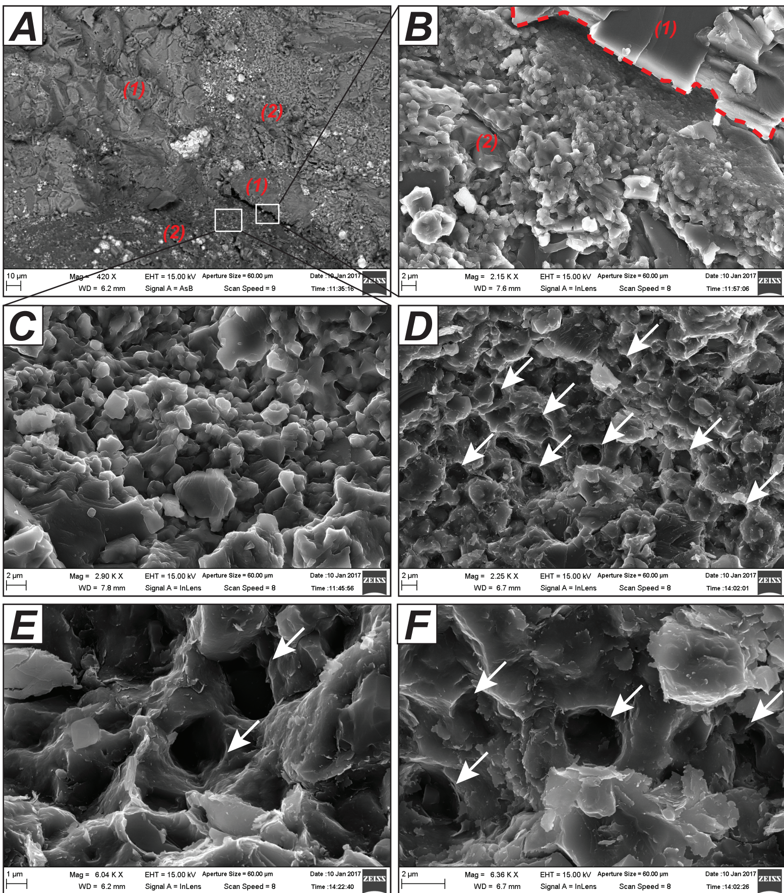
Figure 4 : A - Cobourg limestone layout with boundary between the two microtexture phases : (1) the main calcite phase and (2) the calcite-clay phase. B - Close-up of the microtexture boundary of picture A. C - Matrix layout of the calcite-clay area. D, E & F - Well-developed microporosity framework in calcite-clay part, with small rounded pores (1-2 \mu\text{m} , white arrows).
