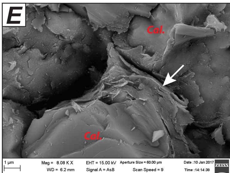
Figure 2 : A - Crack-like pores located at calcite crystal boundaries (white arrows). B - close-up of picture A, microcrack-like pores in a calcite crystal (white arrows). C, D, E & F - Matrix layout of the calcite phase with clay-flakes (white arrows) located at crystal boundaries, and coating crystal ( Cal. ) edges.
