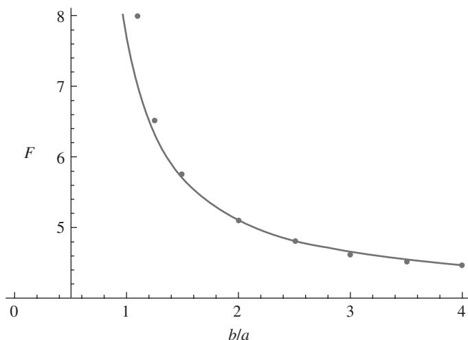
Figure 5. Influence of the geometry of the sealing patch on the intake shape factor (the solid line indicates the result obtained from equation (3.23)). The dots indicate results due to Goggin et al. (1988) and Tartakovsky et al. (2000).
