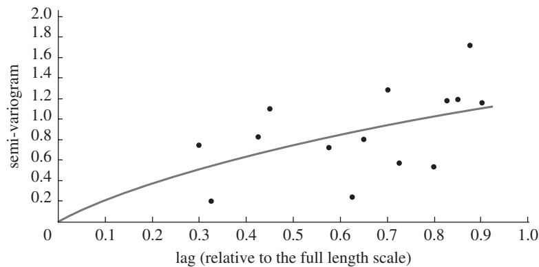
Figure 11. The exponential Bessel theoretical semi-variogram (grey) based on an experimental semi-variogram (black).
