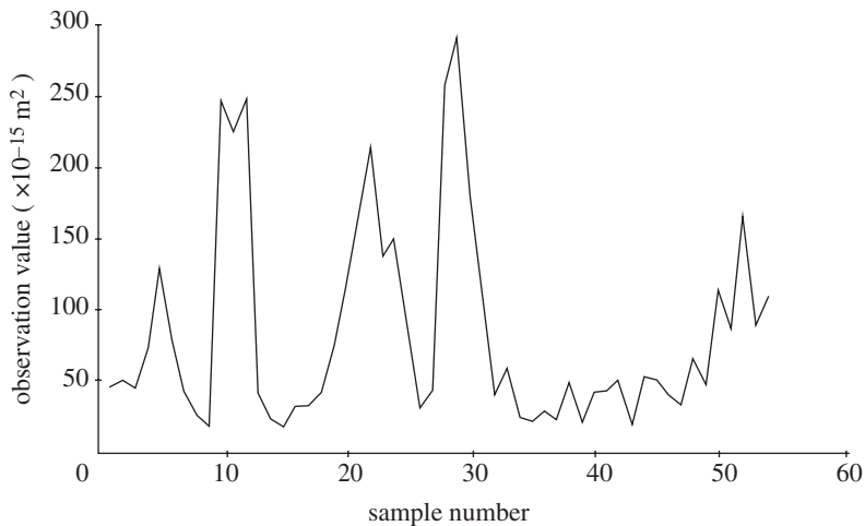
Figure 10. Initial data points (from table 1) sampled by EASYKRIG v.3.0.
