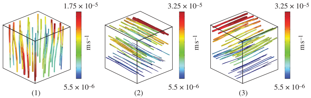
Figure 14. Stream tube patterns along three orthogonal directions.
