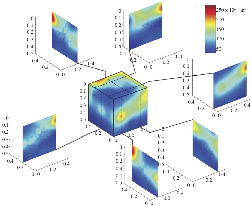
Figure 12. Distributions of permeability within the Indiana limestone block as estimated by kriging the experimental data obtained from surface permeability measurements.
