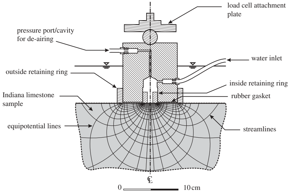
Figure 1. Details of the permeameter.
