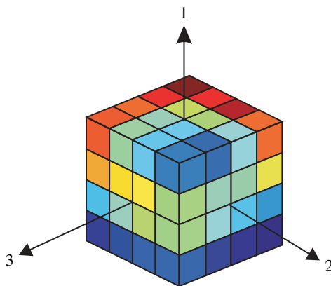
Figure 13. A substructured unit of the cuboidal sample of Indiana limestone with permeabilities derived from the kriging procedure.
