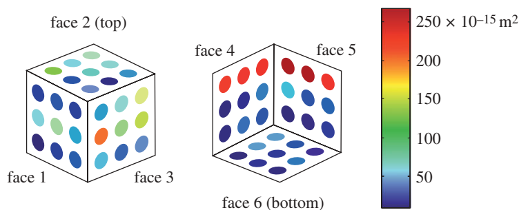
Figure 9. Preliminary distributions of permeability corresponding to the test data shown in table 1.
