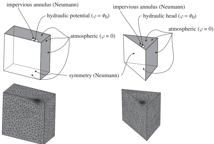
Figure 7. Computational modelling for fluid flow associated with the permeameter located either along the edge or at the corner of the cuboidal specimen.
