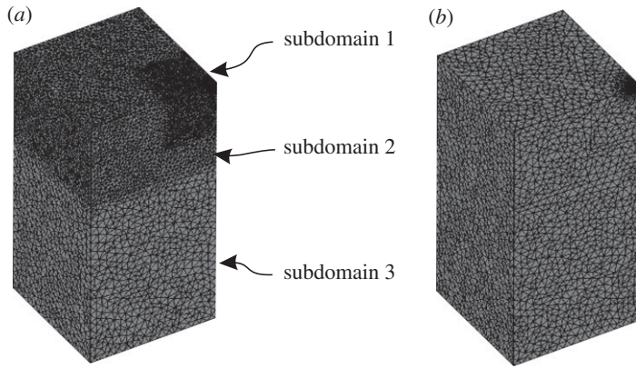
Figure 6. (a,b) Finite-element discretizations of the flow domain.
